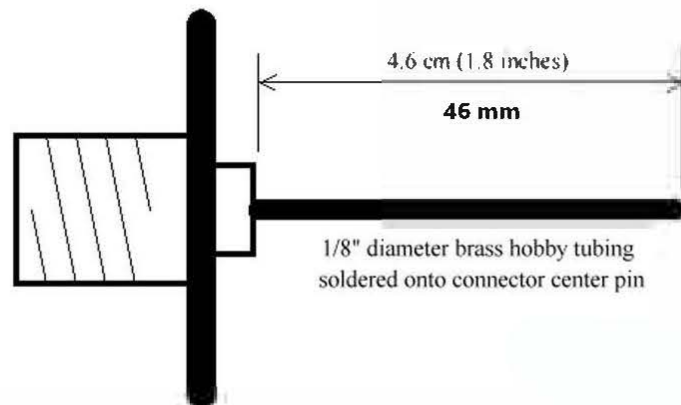
Type N Female Flange Mount Coaxial Connector
