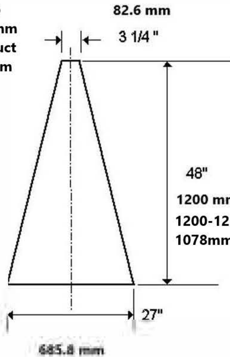
Horn Side Panels
