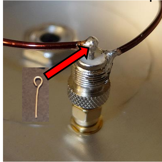
F-type <> SMA Adapter soldered to 21cm circumference wire loop
