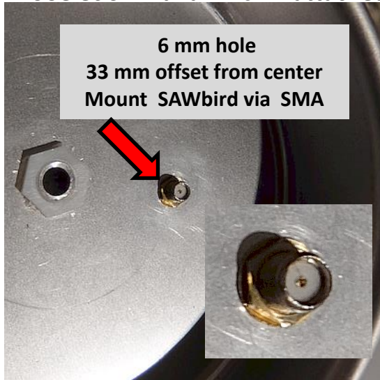
noelec SAWbird H1 SMA attached to 6" dia x 2" deep Cake Pan
